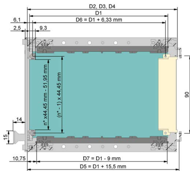
Side view, standard
